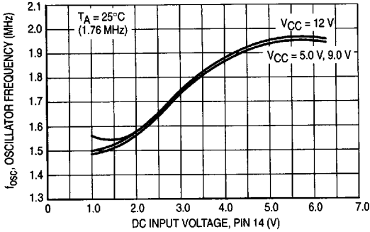
Figure 13. Modulator Transfer Function
