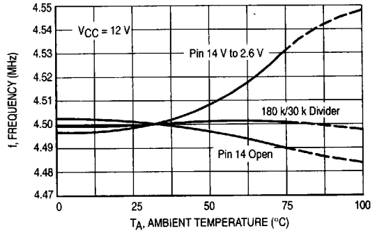
Figure 16. FM System Frequency versus Temperature
