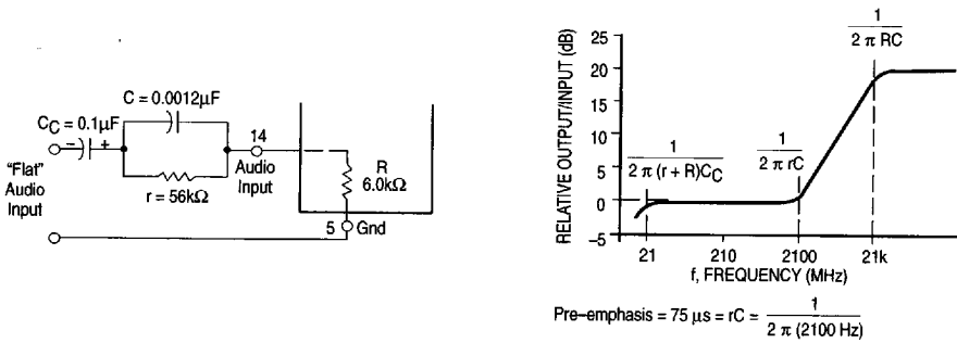
Figure 20. Audio Pre-Emphasis Circuit
