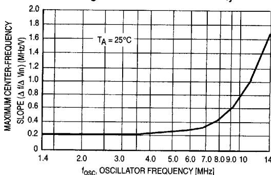
Figure 12. Modulator Sensitivity
