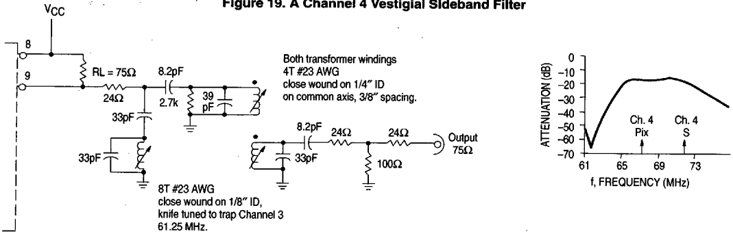
Figure 19. A Channel 4 Vestigial Sideband Filter
