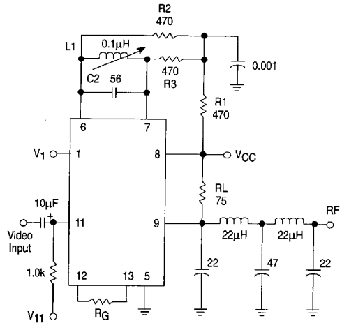
Figure 4. AM Test Circuit
