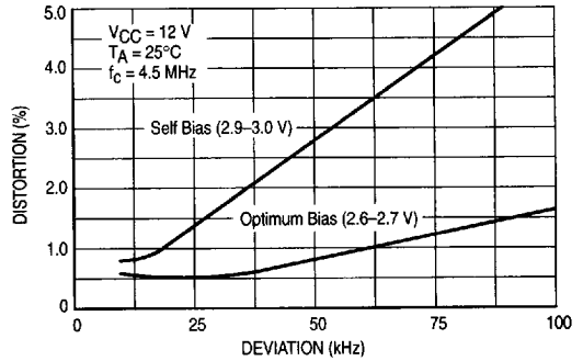
Figure 14. Distortion versus Modulation Depth
