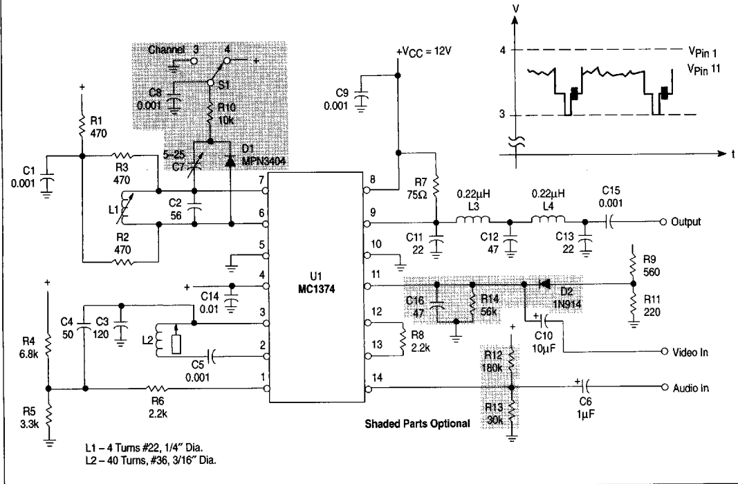
Figure 1. Simplified Application
