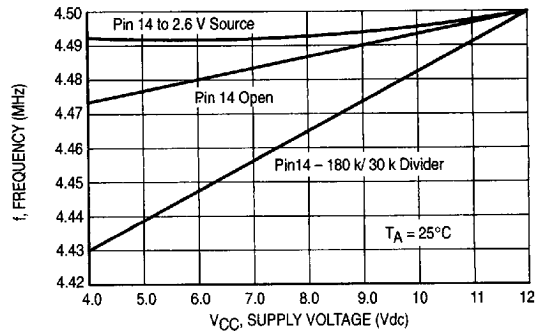
Figure 18. FM System Frequency versus V_{CC}
