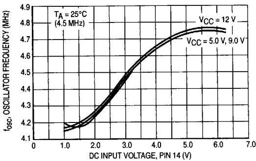
Figure 15. Modulator Transfer Function
