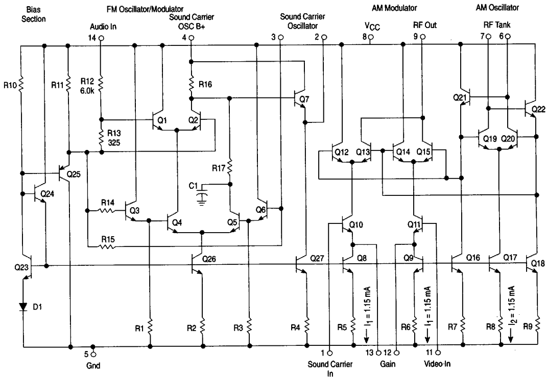
Figure 2. TV Modulator
