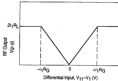
Figure 3. AM Modulator Transfer Function
