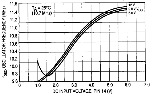
Figure 17. Modulator Transfer Function
