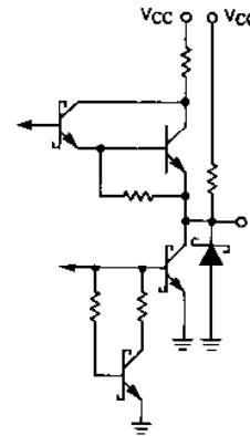
FIGURE 24 — TYPICAL INPUT
