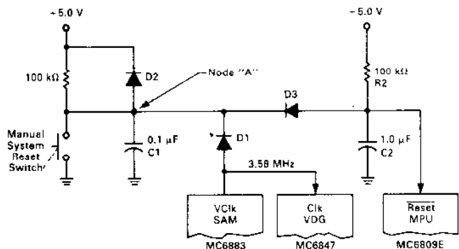
FIGURE 7 — EXTERNAL RESET CIRCUITRY
