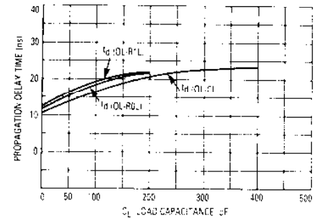
FIGURE 1 — PROPAGATION DELAY TIMES VERSUS LOAD CAPACITANCE
