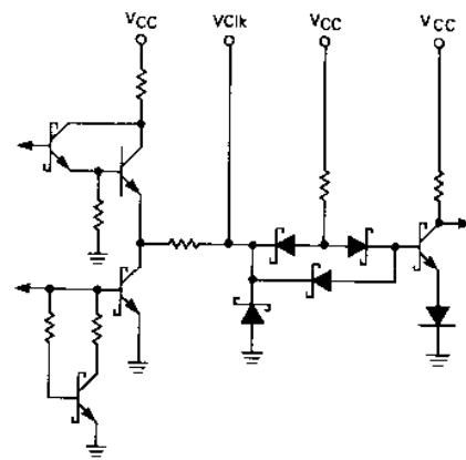
FIGURE 22 — VClk INPUT/OUTPUT
