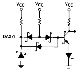
FIGURE 21 — DA0 INPUT
