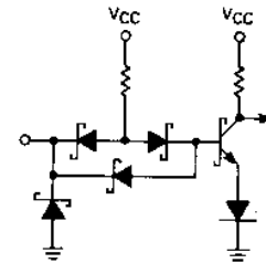
FIGURE 25 — TYPICAL OUTPUT
