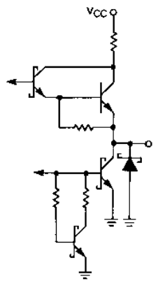
FIGURE 25 — TYPICAL OUTPUT
