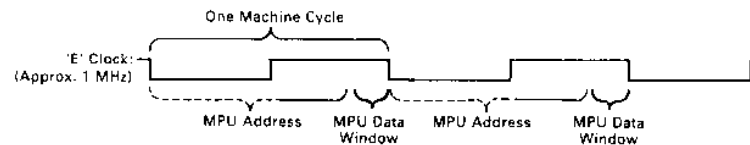
FIGURE 11 — MOTOROLA MPU TIMING
