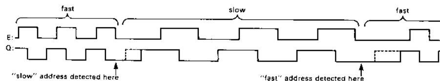
FIGURE 8 — RATE CHANGE E AND Q WAVEFORMS
