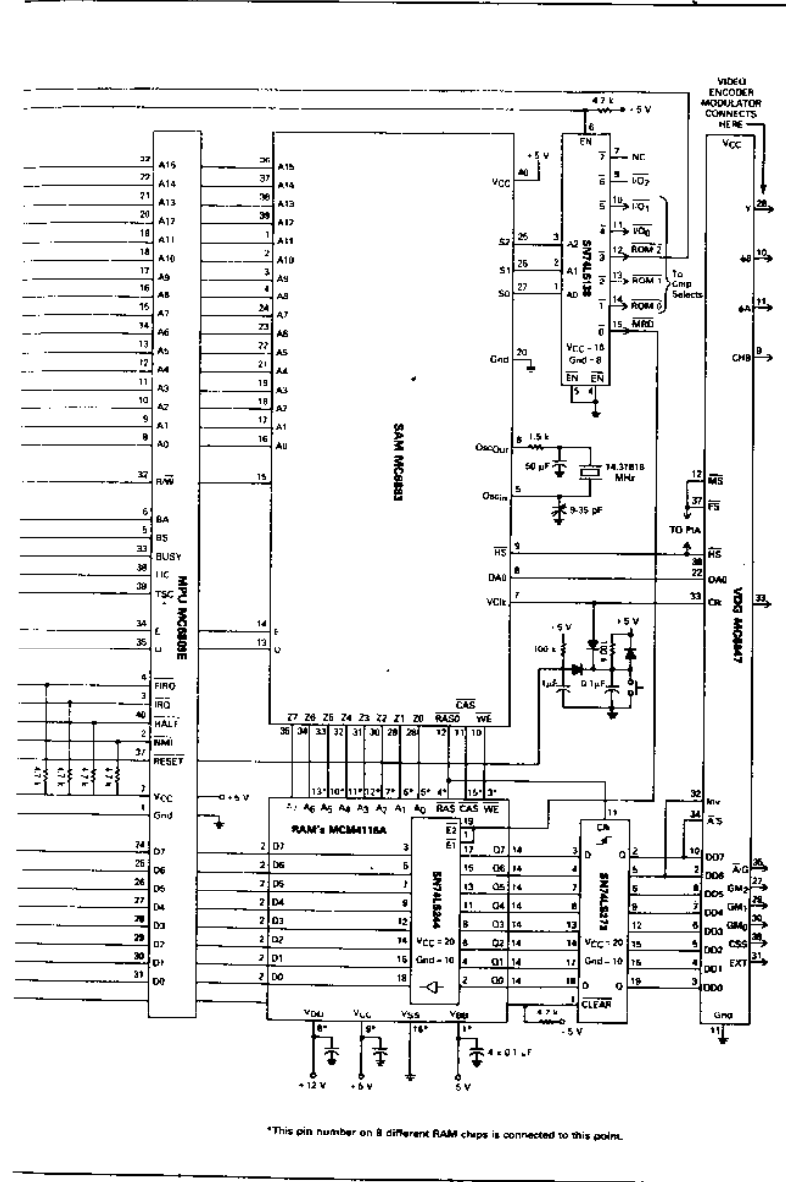
FIGURE 19 — EXAMPLE of MC6809E, MC6883 and MC6847 COMPUTER
