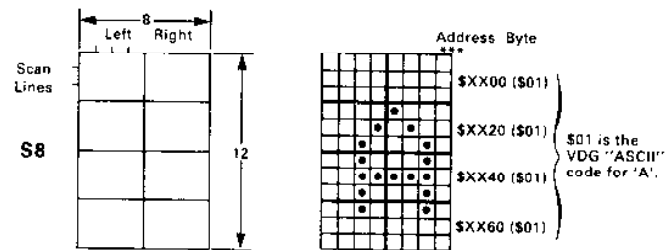
FIGURE 17 — DISPLAY MODES S8, S12, S24 Bit/Visible Dot Correlation
