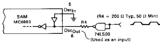
FIGURE 10 — TTL CLOCK INPUT
