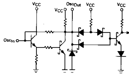
FIGURE 20 — EQUIVALENT OF OSCILLATOR INPUT AND OUTPUT
