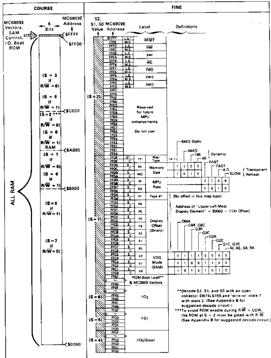
FIGURE 15 — MEMORY MAP (TYPE #1)
