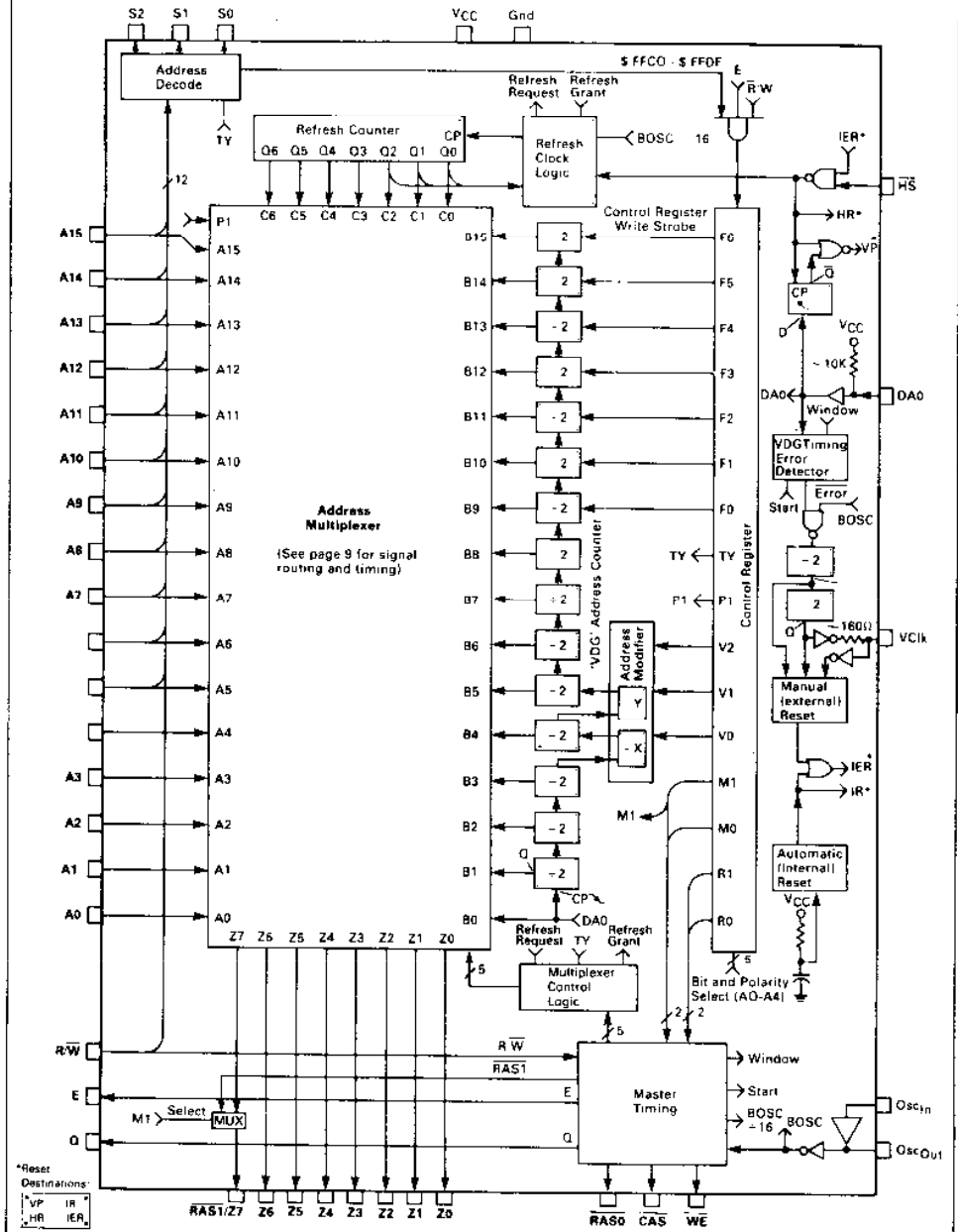
FIGURE 4 — SAM BLOCK DIAGRAM
